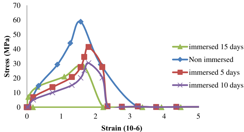
Figure 6. Tensile Strength of glass kenaf hybrid composite.
