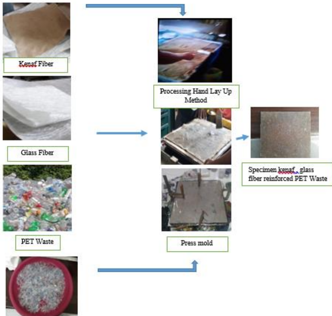
Figure 2. Composite manufacturing procedures.
